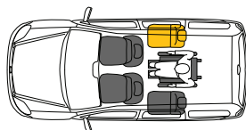
Freewheeler Caddy Life 5 passenger layout
